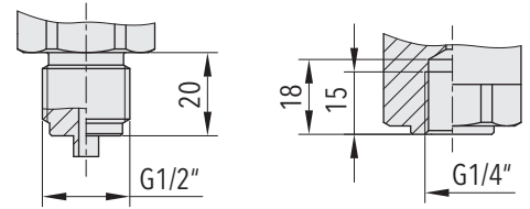
G1/2" male
