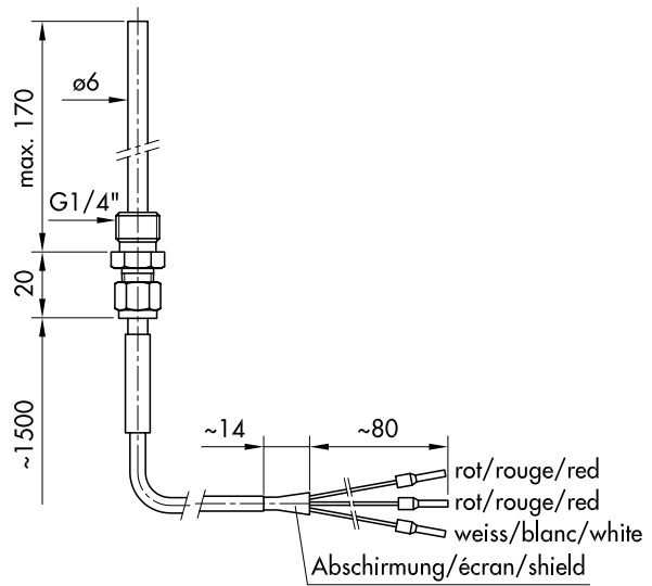
XXXX.XX.1013.XX 0...550°C
